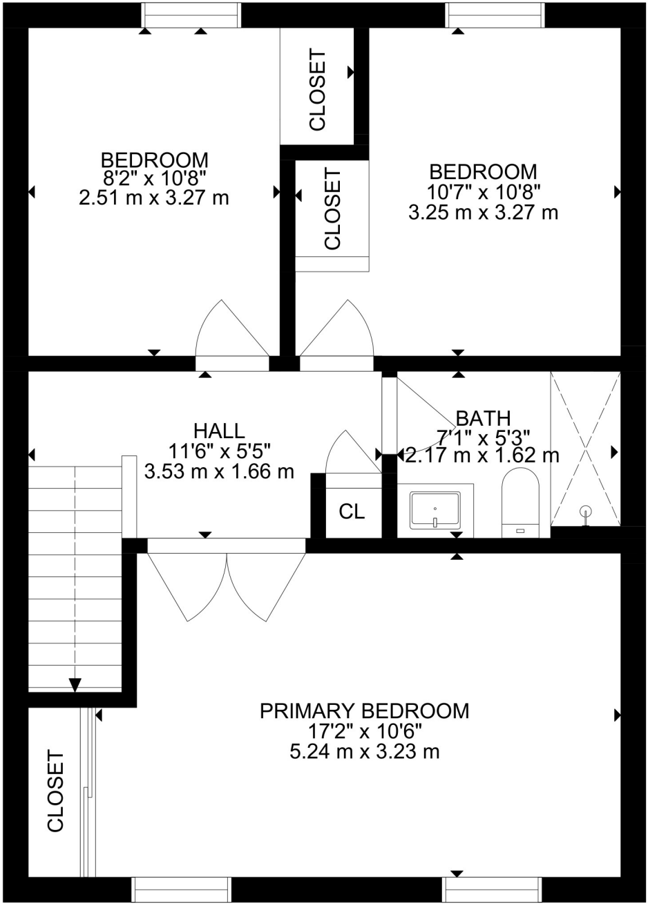
UPPER FLOOR
