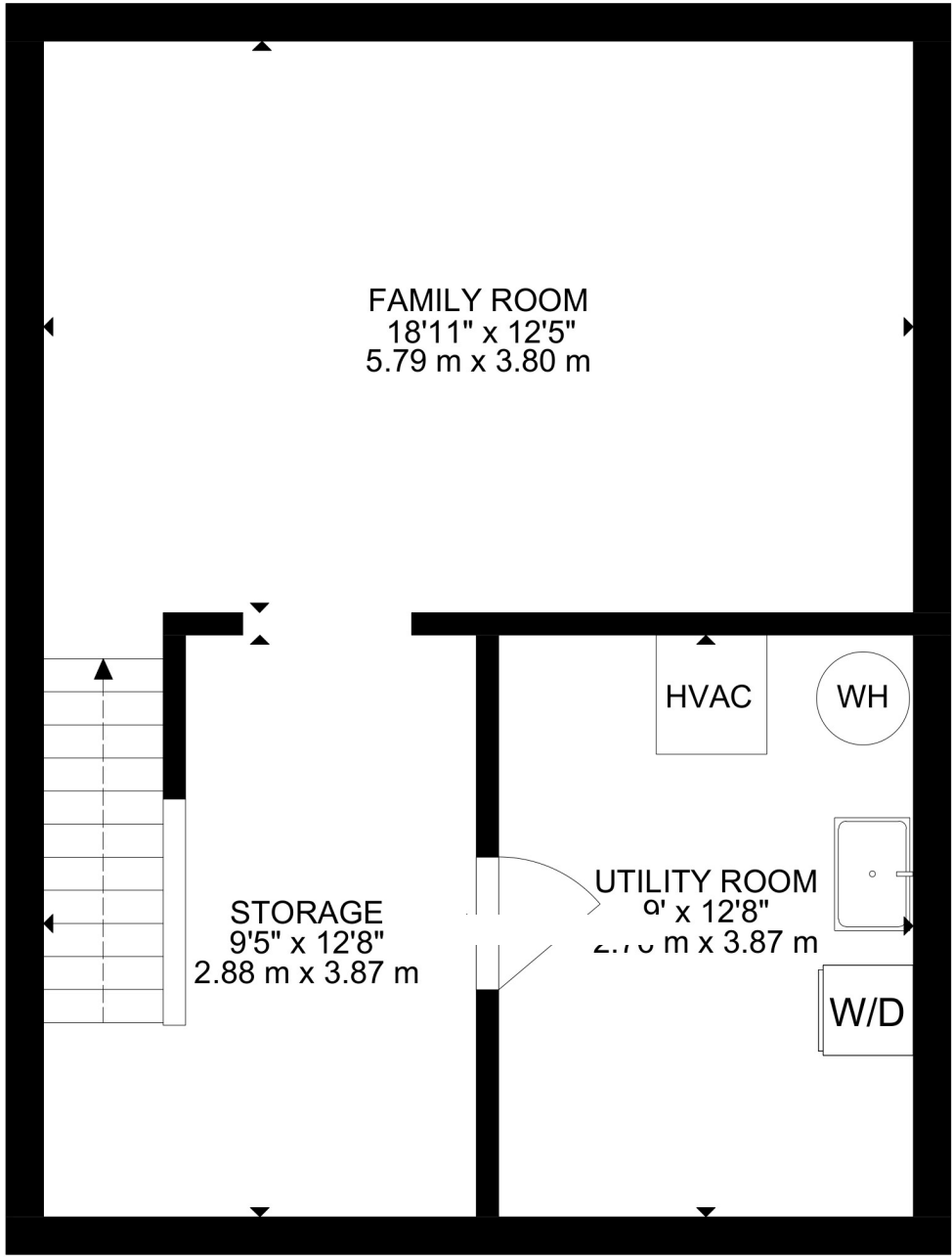
LOWER FLOOR
