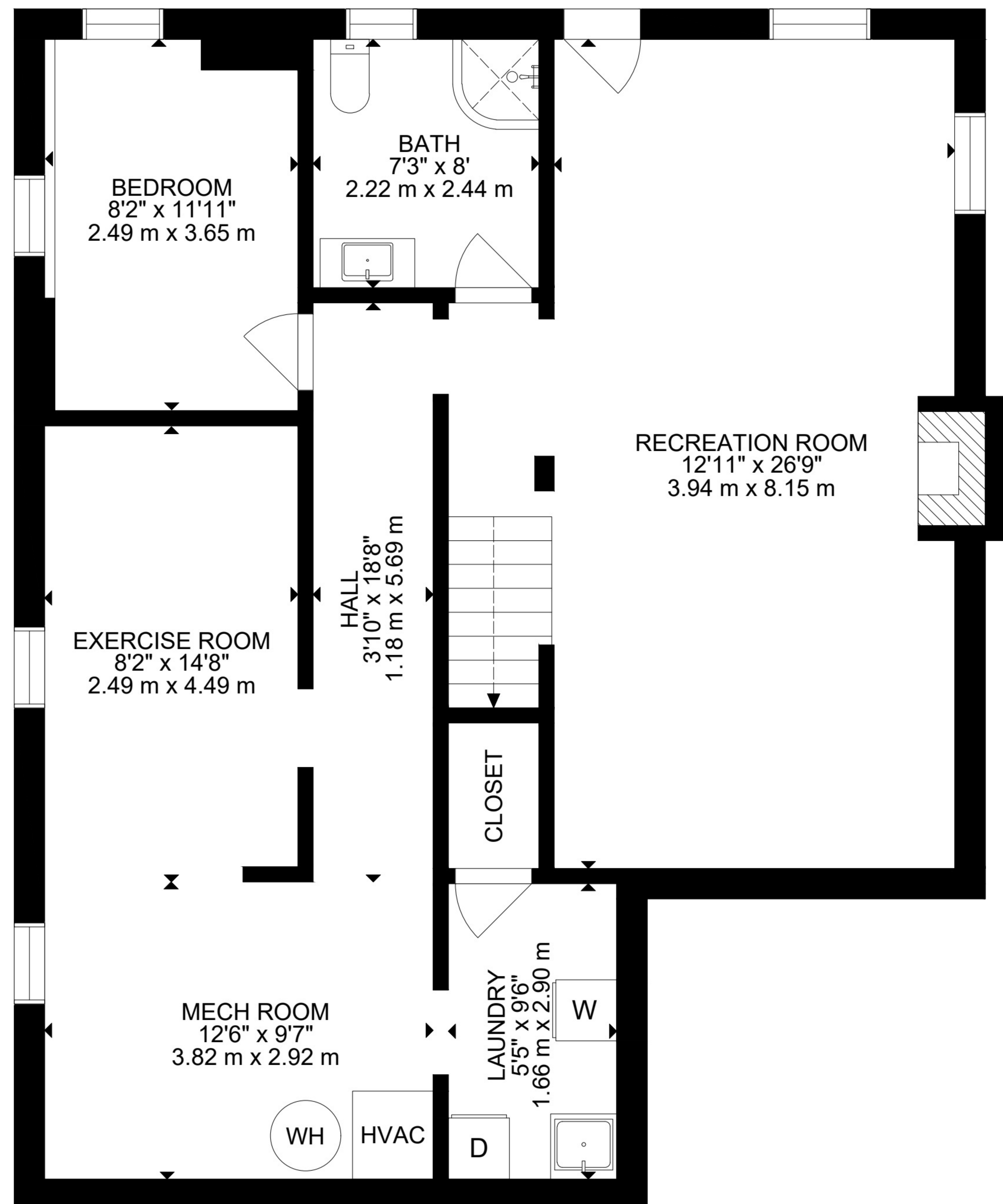
LOWER FLOOR
