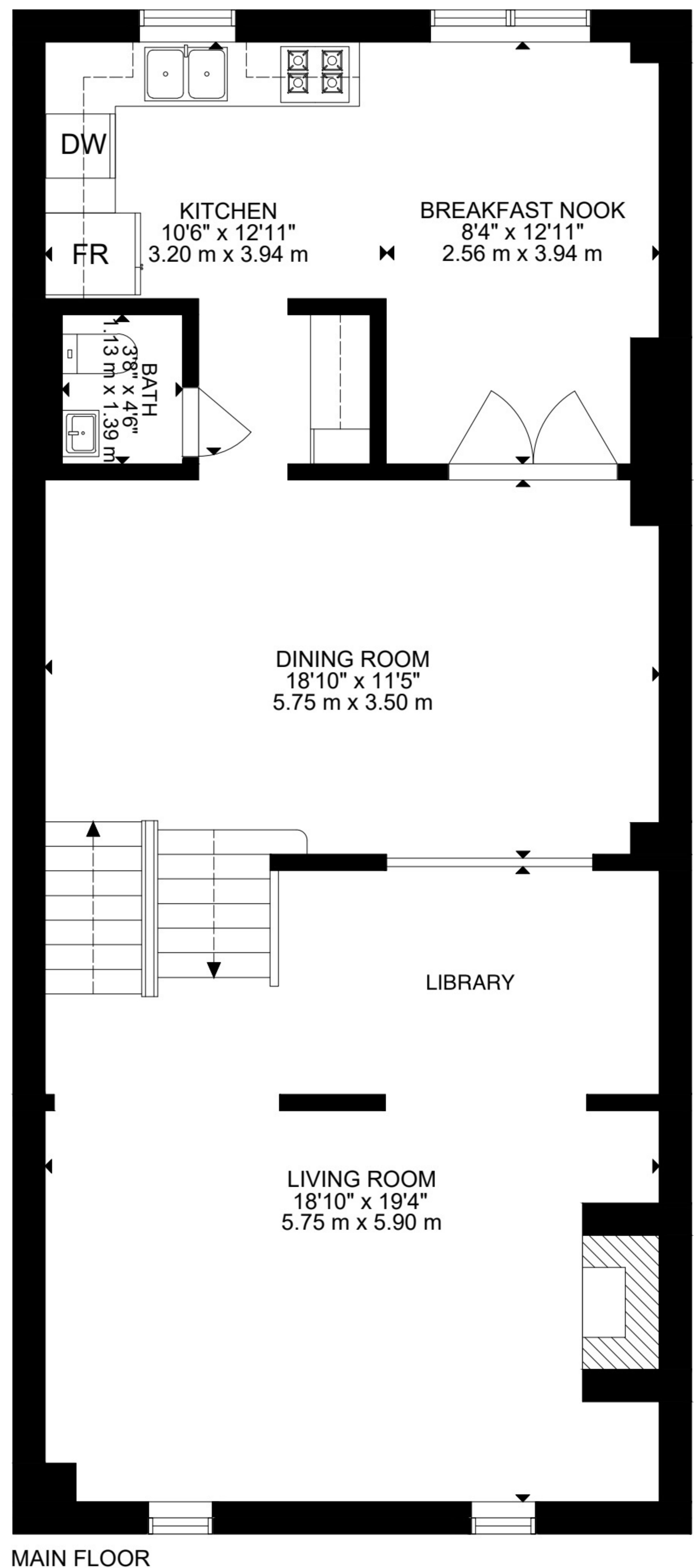
MAIN FLOOR
